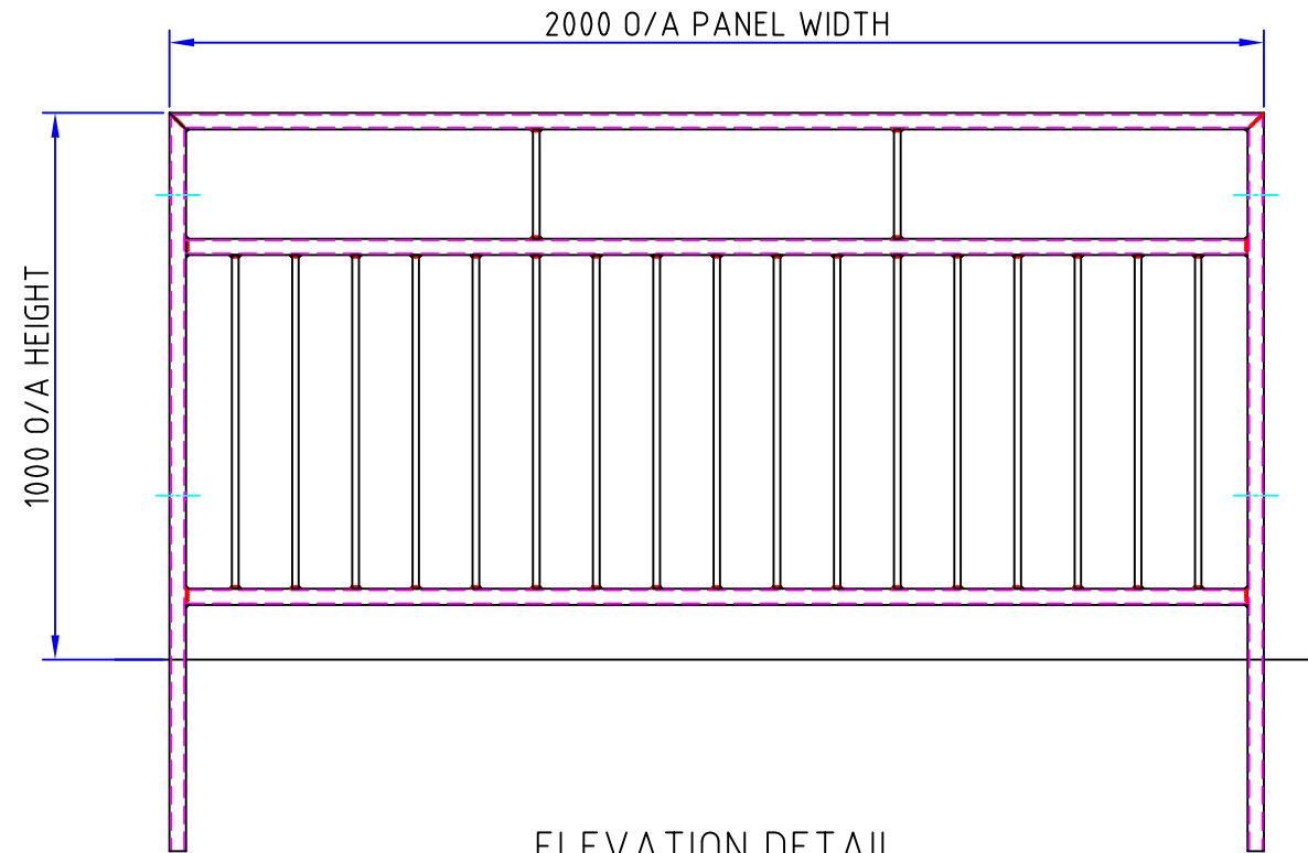
ELEVATION DETAIL PED-GUARD RAIL PANELS c/w VISIBILITY GAP
