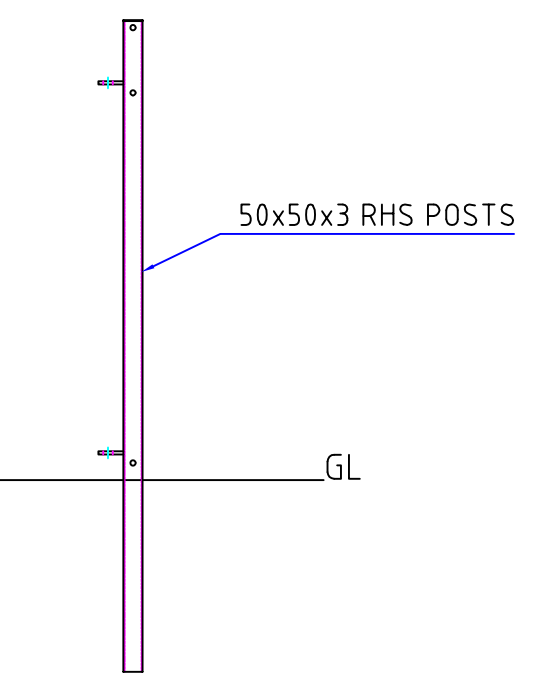
TYPICAL LOOSE CLEAT POST ELEVATION
