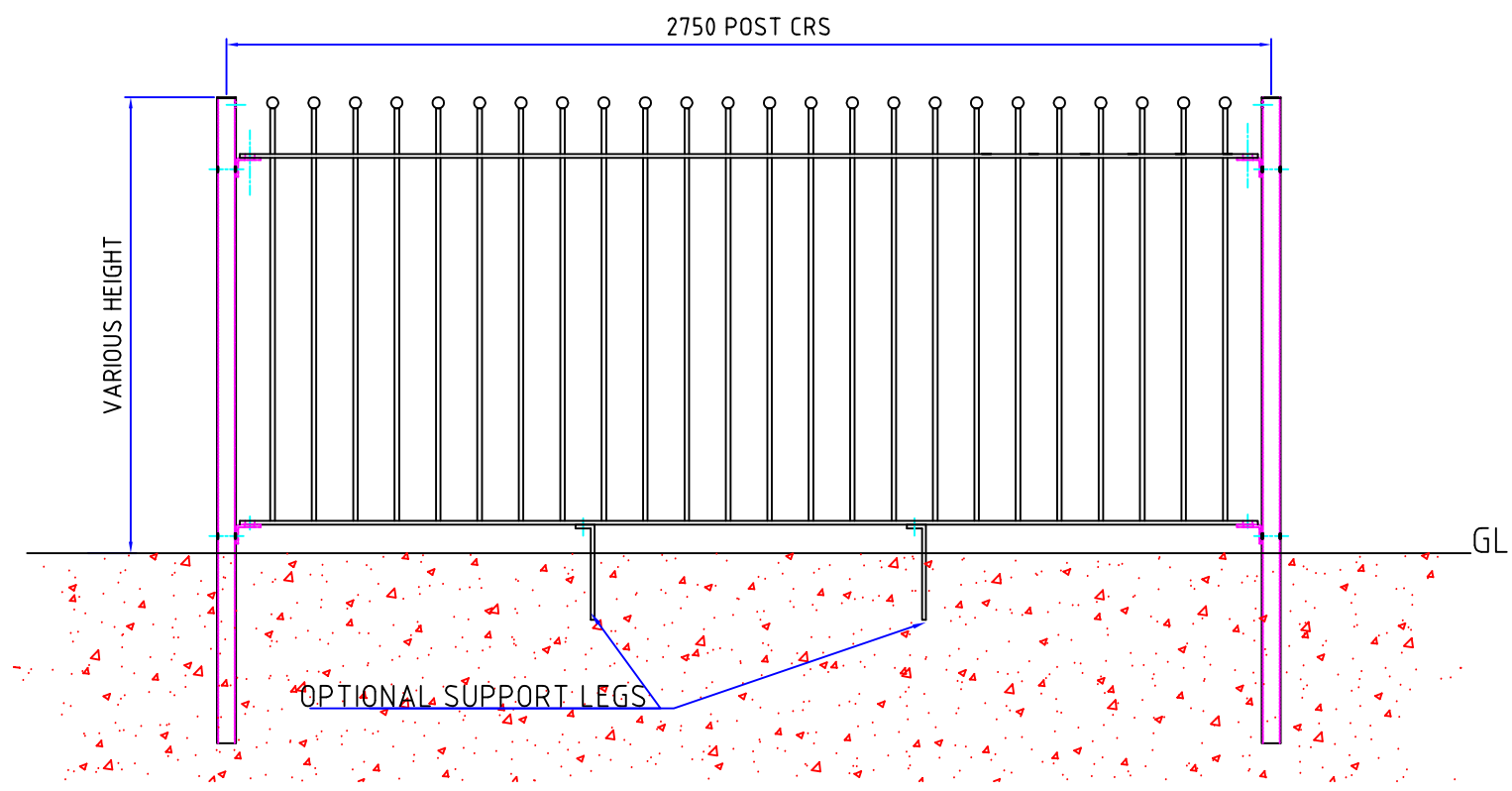
TYPICAL PANEL ELEVATION
