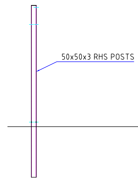
TYPICAL LOOSE CLEAT POST ELEVATION
